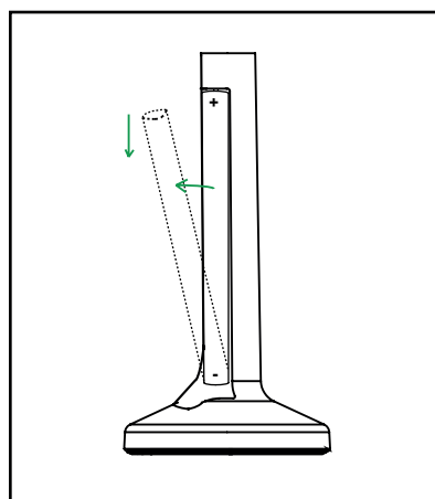
fase 5: remove the battery. Push the battery down before pulling out. Attention: The device must be switched off before removing the battery.
